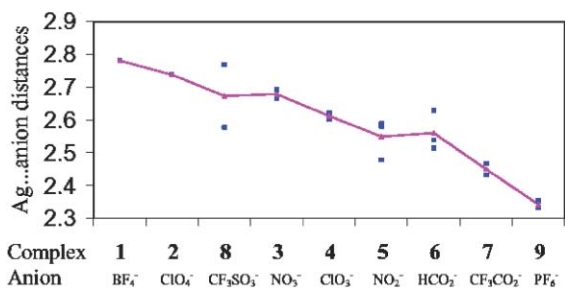
Chart 1 Trend of Ag...anion distances (Å) in complexes 1–9 based on the structural data listed in Table S1. A line is drawn through the weighted average values.
